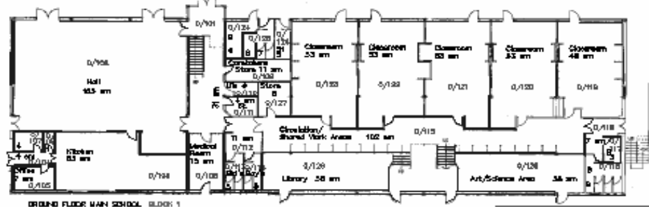
GROUND FLOOR MAIN SCHOOL BLOCK 1
